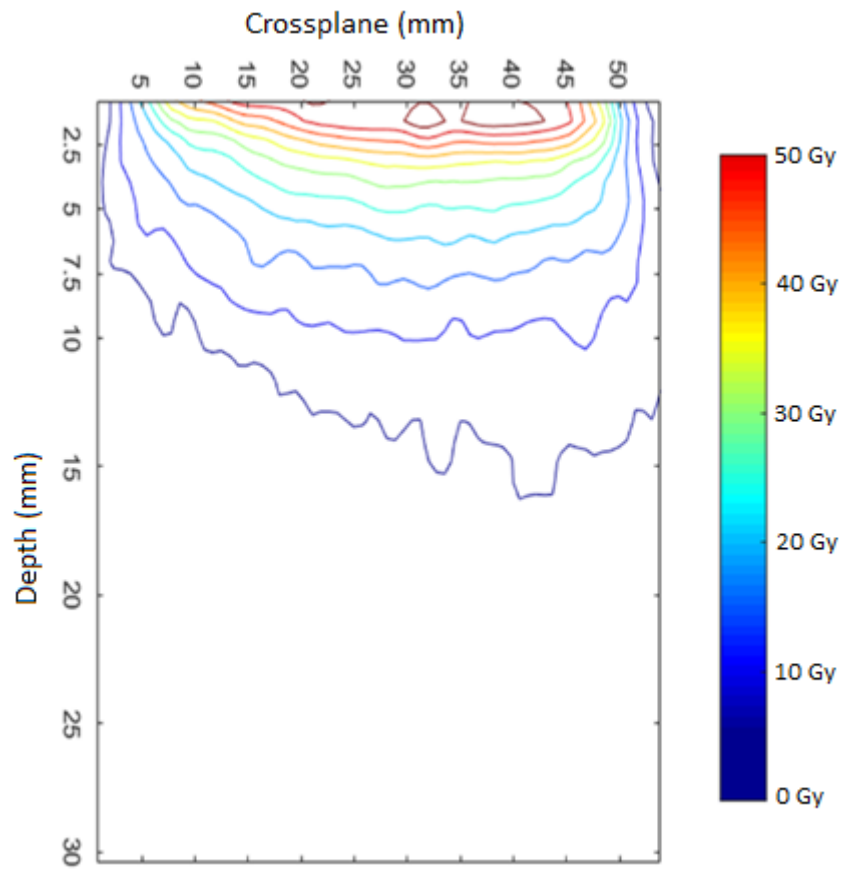
Figure 1: isodose map for an irradiated gel at 50 Gy
